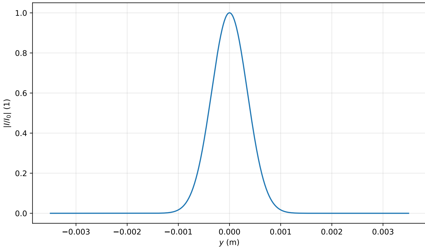
Intensity profile I(x = 0, y, z = 0.080)/I_0 , P_{in}=0.3P_{cr} , artificial time
